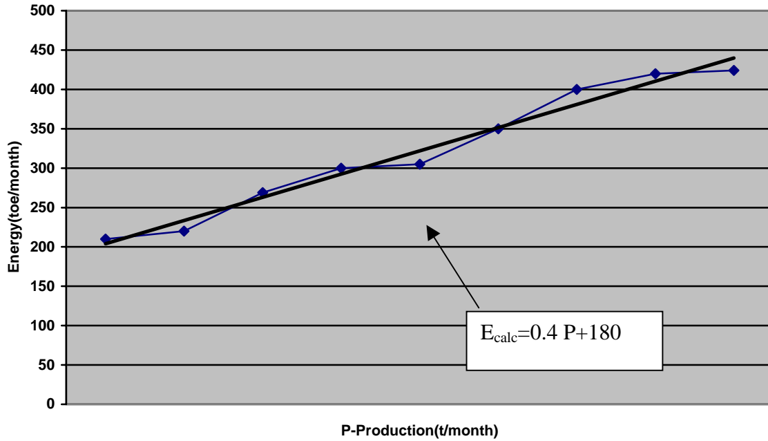
Figure 8.9 Energy Production Graph
