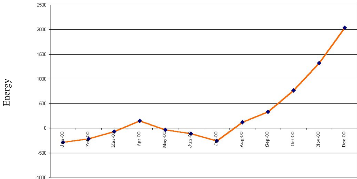
Figure 8.8 CUSUM Chart
