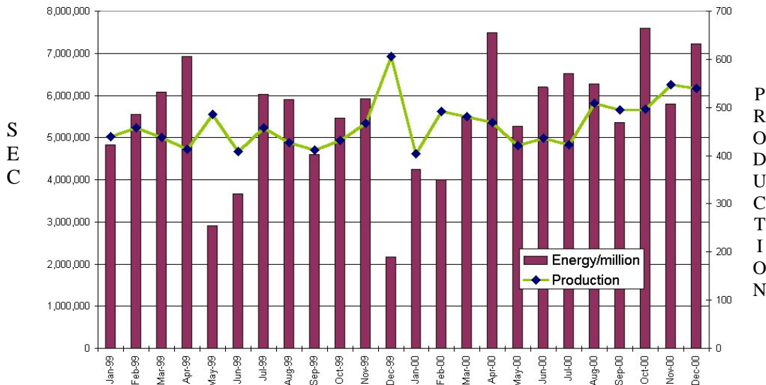
Figure 8.6 SEC With Production
