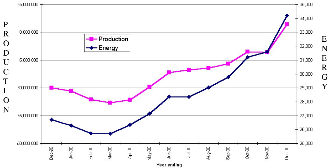
Figure 8.4 Moving Annual Total – Energy and Production
