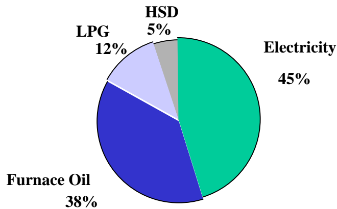
Figure 8.1 % Share of Fuels Based on Energy Bill
