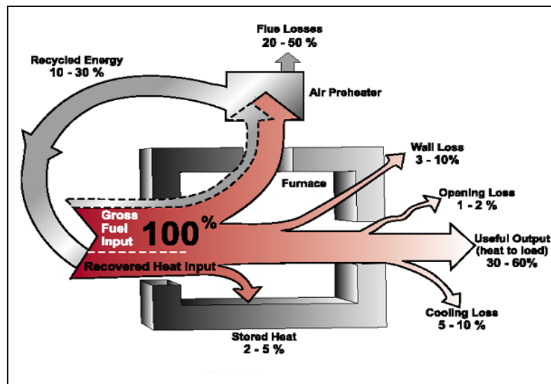
Figure 4.2: Energy Balance for a Reheating Furnace
