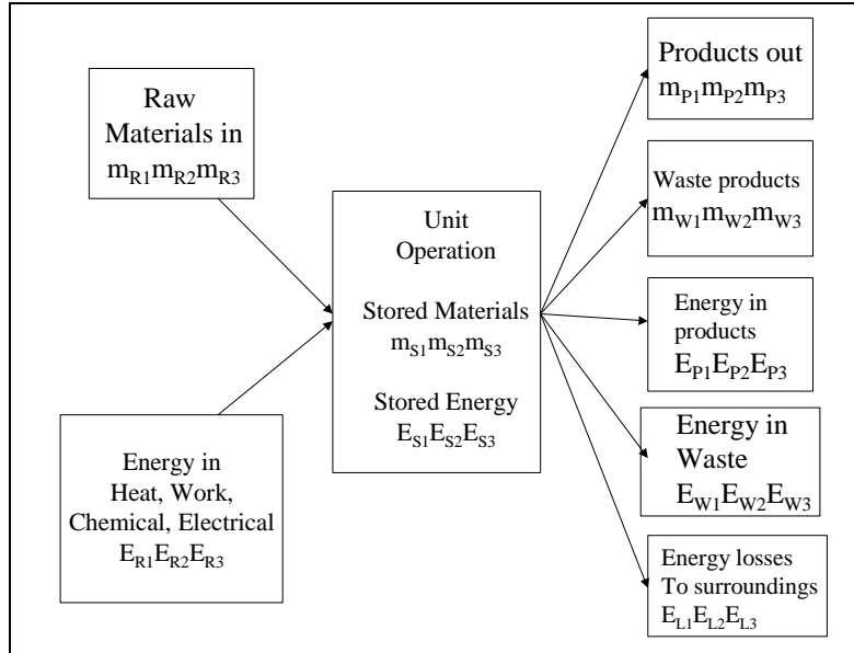
Figure 4.1: Mass and Energy Balance
