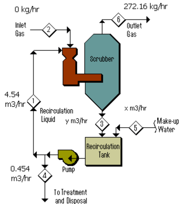
Figure 4.13 Example of Material Balance
